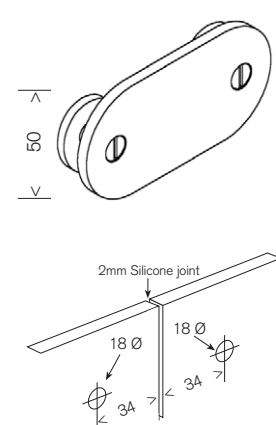
MBR 180D/B 180° Glass to Glass Bracket
