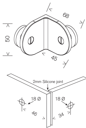
MBR 90D/B 90° Glass to Glass Bracket
