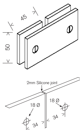
MBS 180D 180° Glass to Glass Bracket
