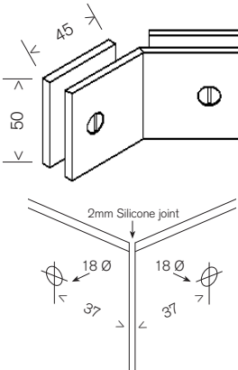
MBS 135D 135° Glass to Glass Bracket
