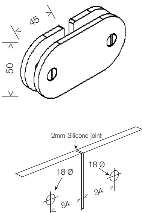
MBR 180D 180° Glass to Glass Bracket
