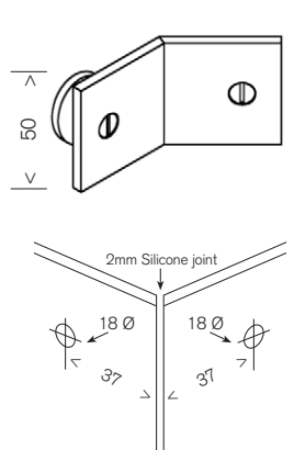
MBS 135D/B 135° Glass to Glass Bracket
