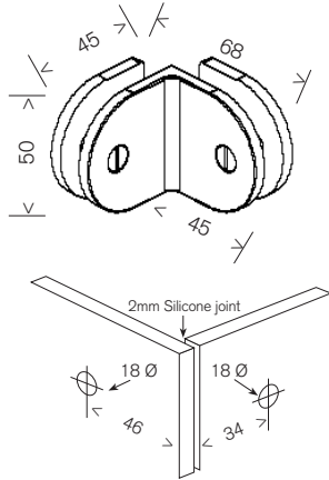
MBR 90D 90° Glass to Glass Bracket
