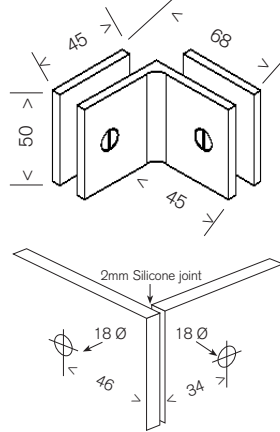
MBS 90D 90° Glass to Glass Bracket
