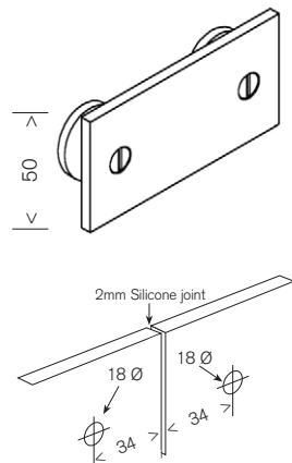
MBS 180D/B 180° Glass to Glass Bracket
