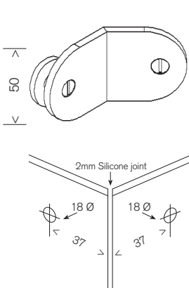
MBR 135D/B 135° Glass to Glass Bracket
