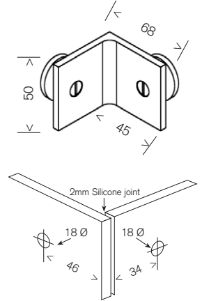
MBS 90D/B 90° Glass to Glass Bracket
