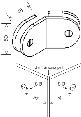
MBR 135D 135° Glass to Glass Bracket
